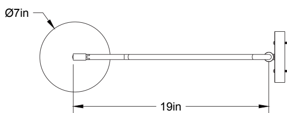
Dessus/Top
